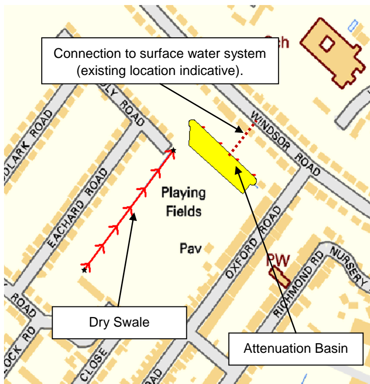
Figure 11-22 Fitzwilliam Playing Fields Attenuation Basin – KH&A-D
