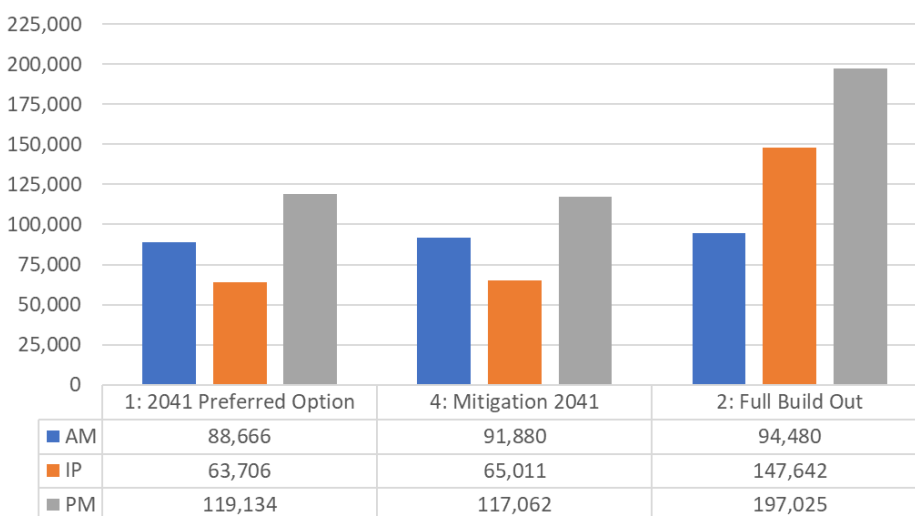
Figure 47 Change in travel distance (PCU-km) vs. 2041 Baseline
