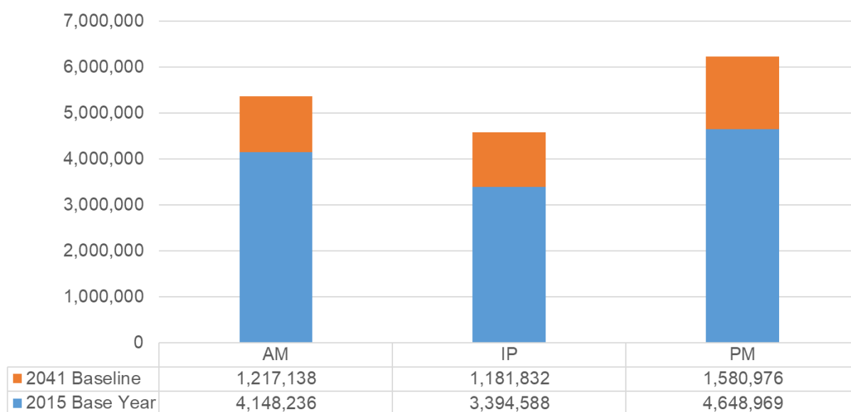
Figure 28 Additional Travel Distance by vehicular traffic (PCU-km) on the Transport Network in the 2041 Baseline over and above the 2015 Base Year
