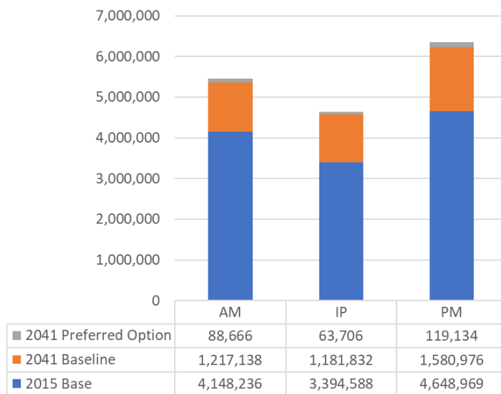
Figure 34 Increase in travel distance (PCU-km) over and above the 2015 Baseline in the 2041 Base Year, and due to the Preferred Option to 2041
