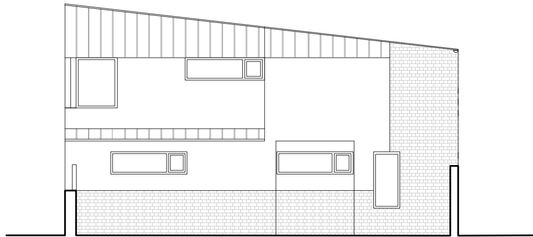
Section C-C
