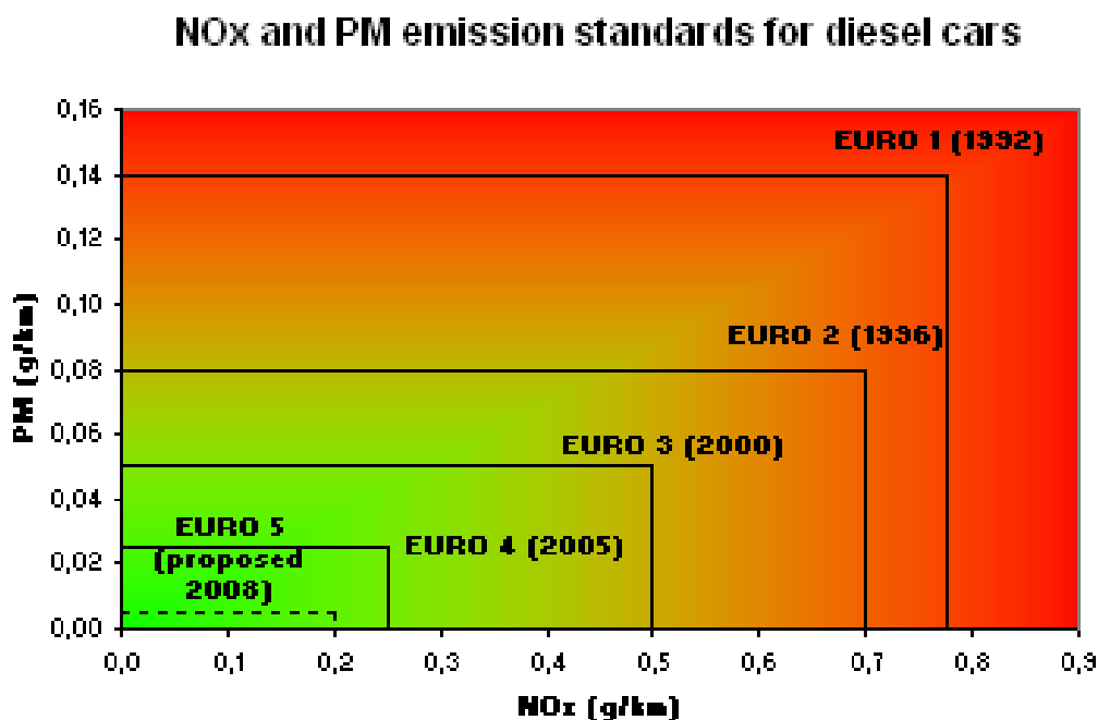
Figure 1 – Chart showing the implementation dates of successive Euro Standards and the No x and PM levels for each of those standards
