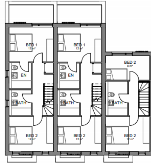
01 - First Floor
